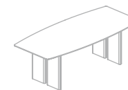
CAS 51 220x100x72 CAS 52 260x120x72
